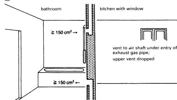
3 Gas space heater in internal bathroom with 'Cologne' ventilation: only permissible if 1 m 3 of space per kW installed is available
